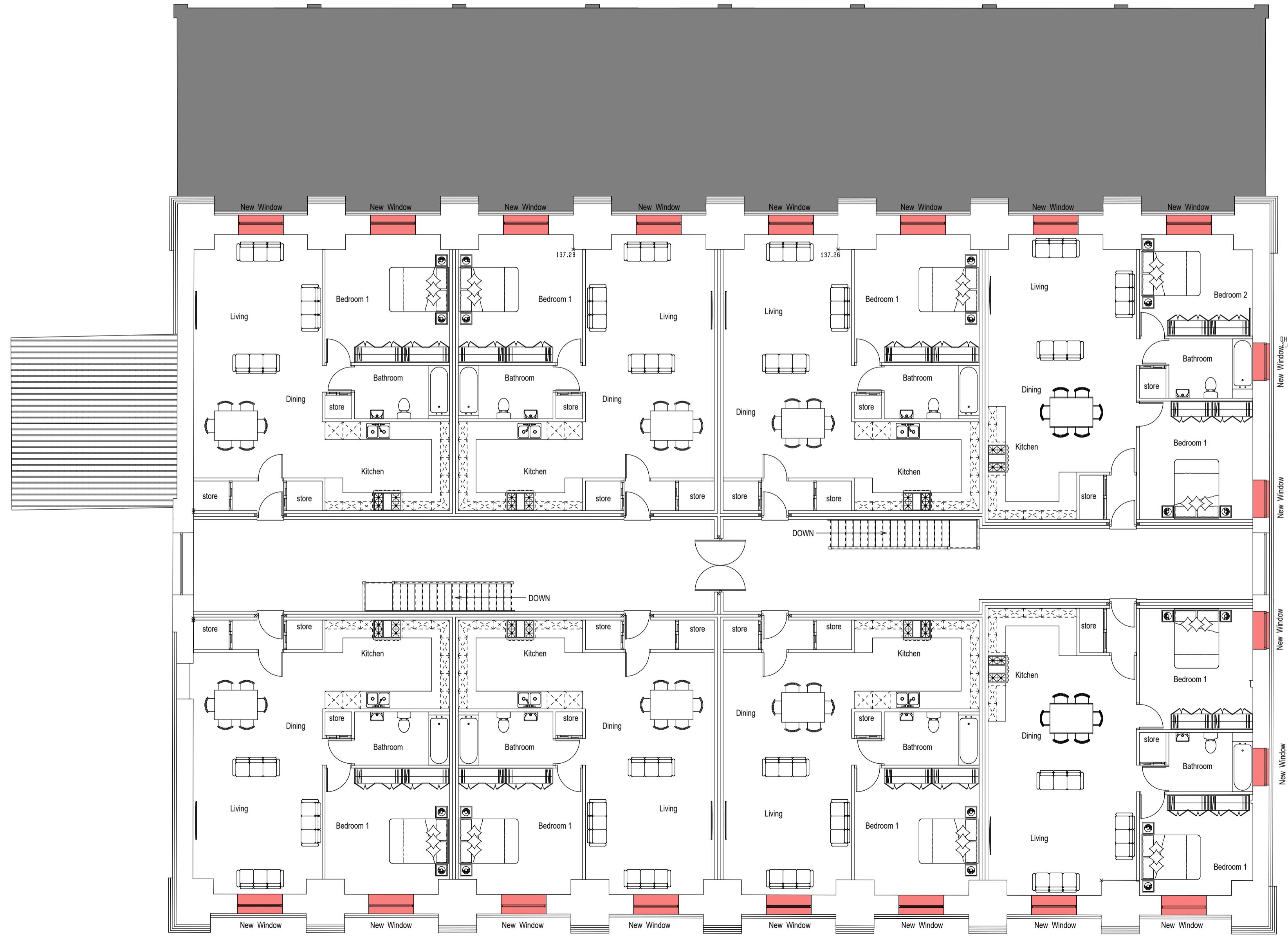
Ground floor
