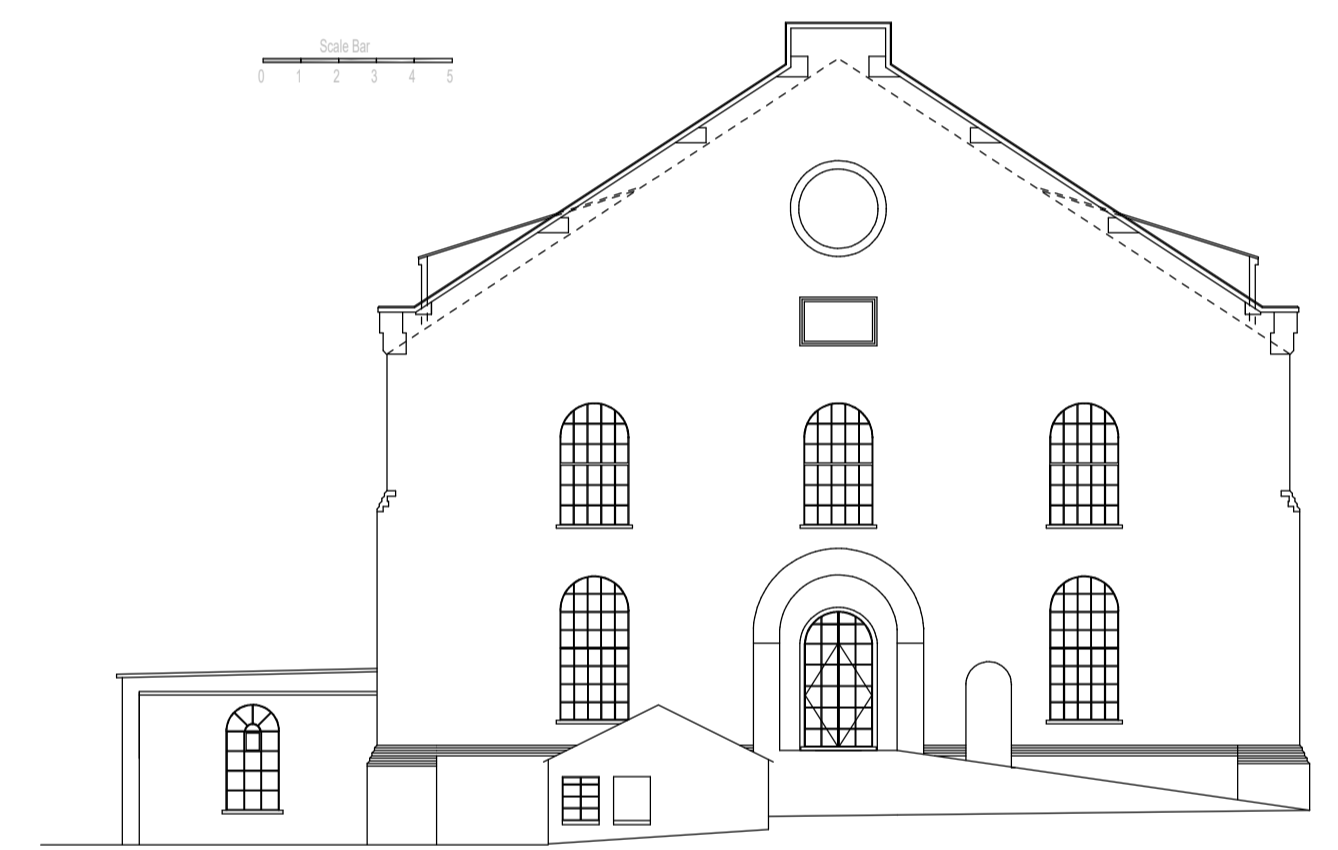
South elevation
