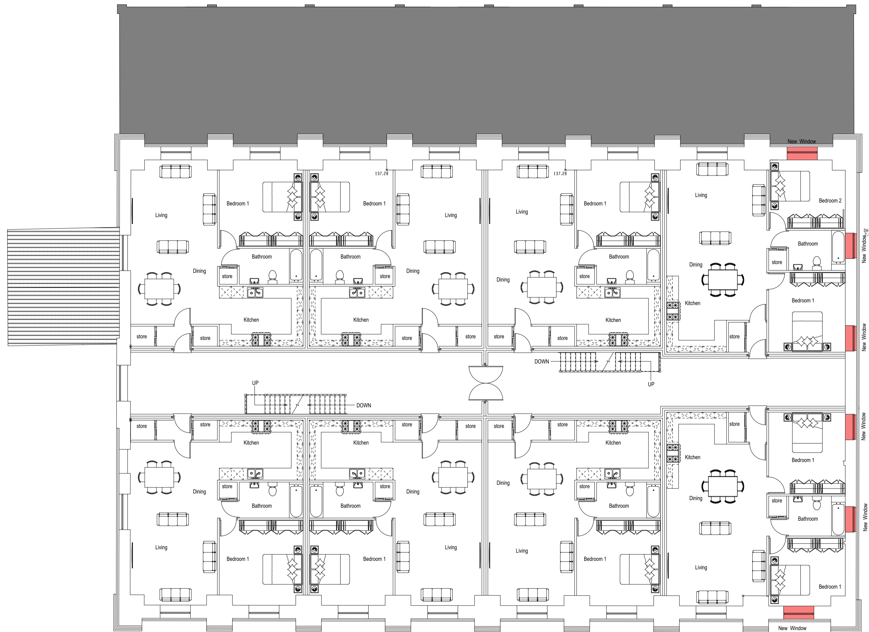
Ground floor
